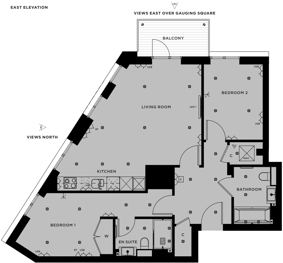
FLOORPLATE
