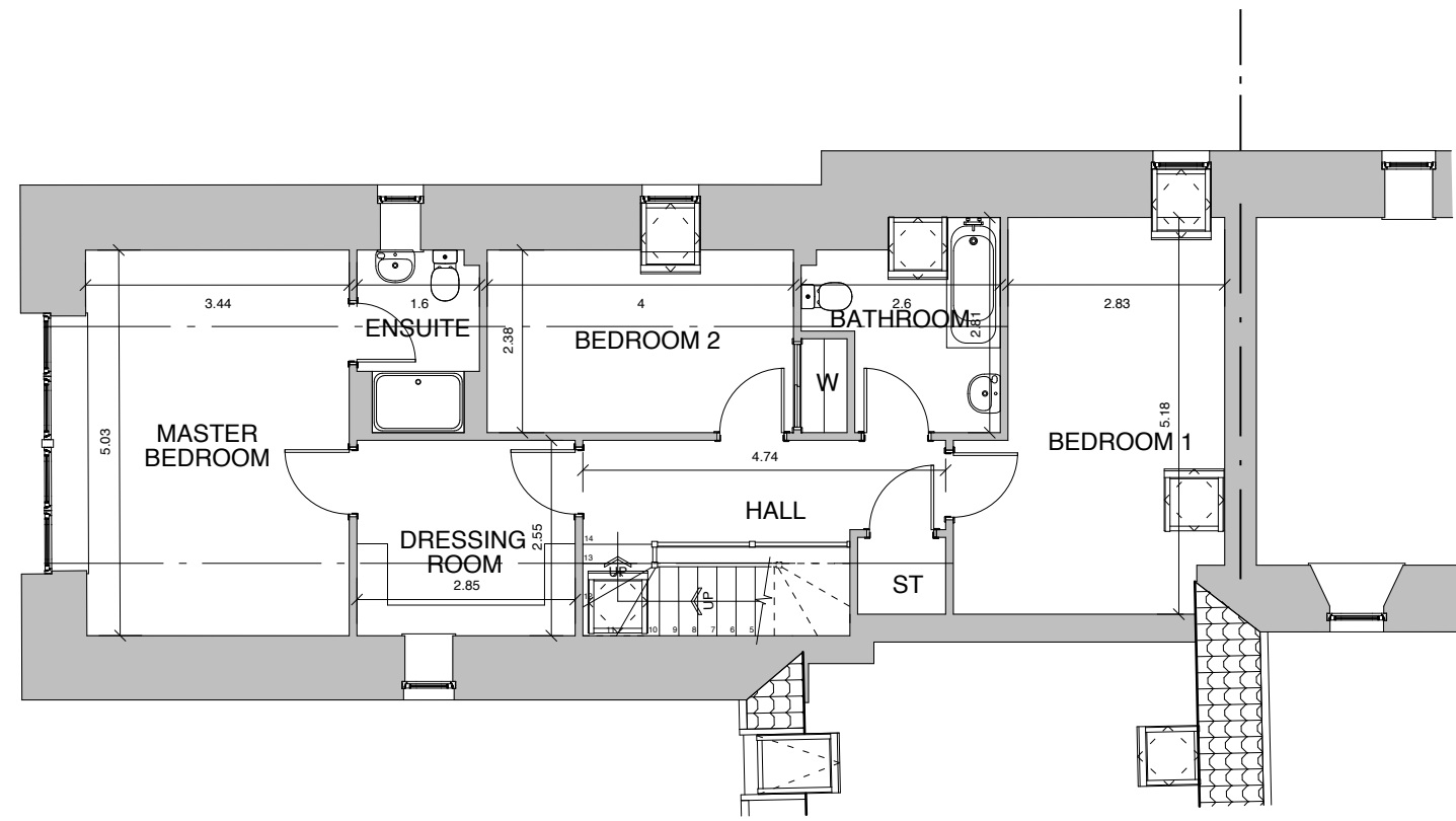
FIRST FLOOR
