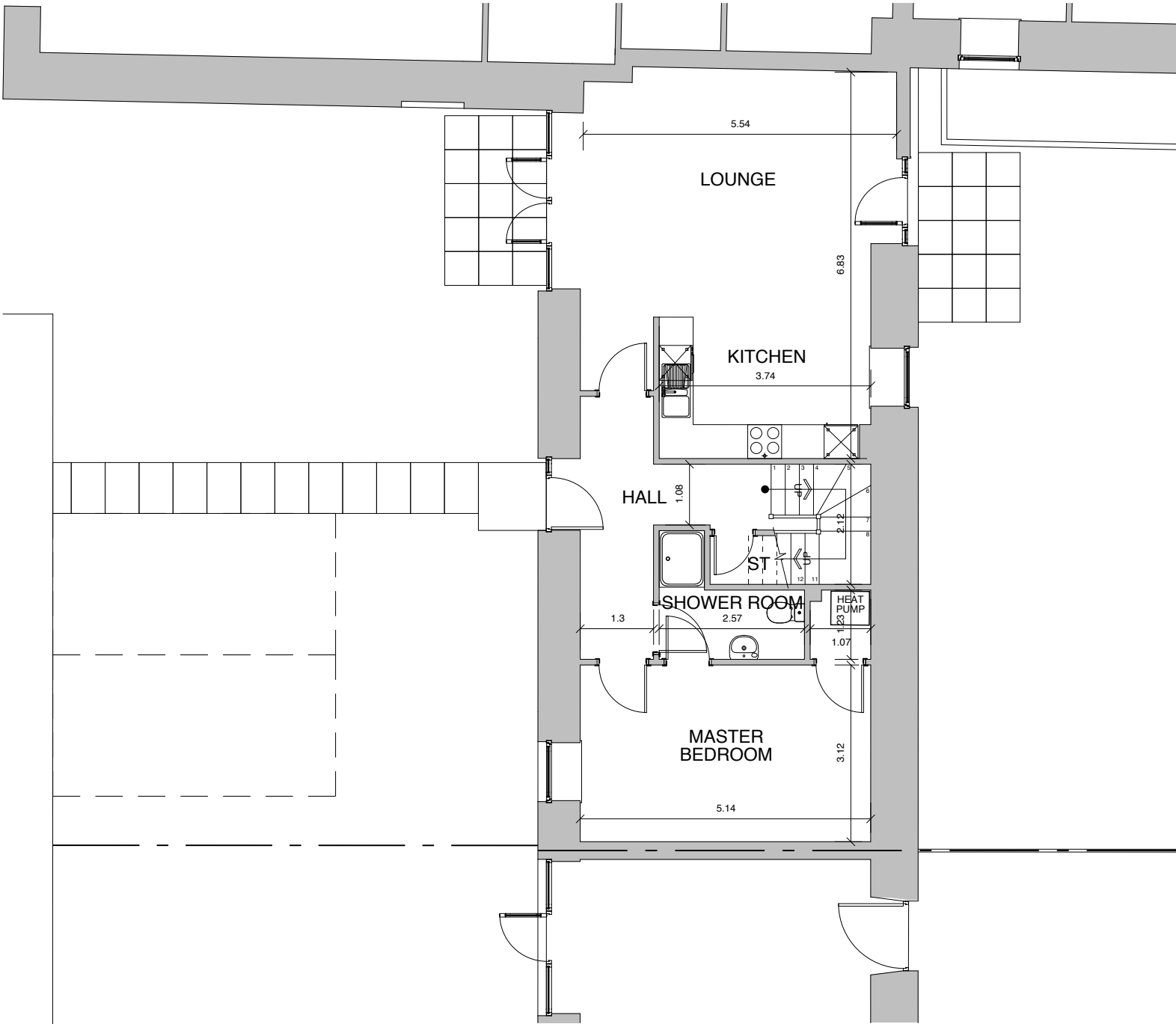
GROUND FLOOR
