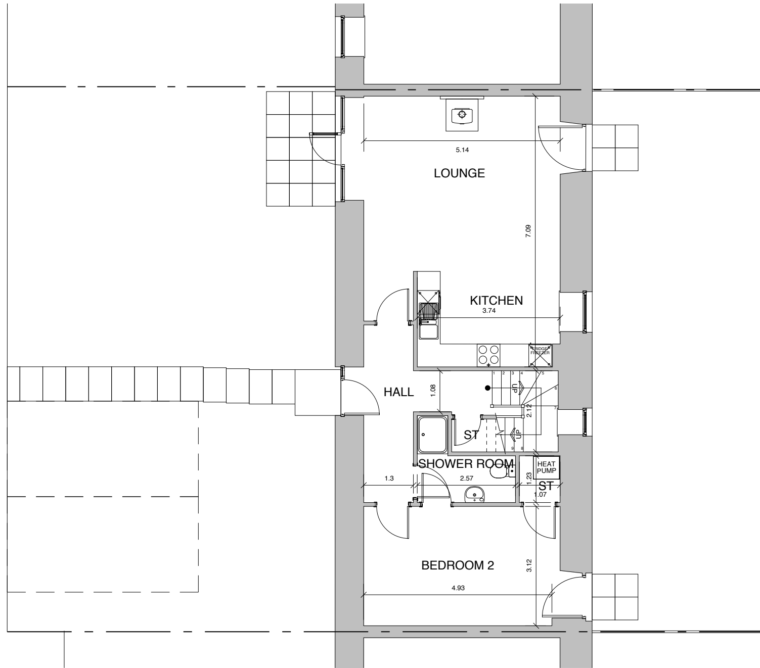
GROUND FLOOR
